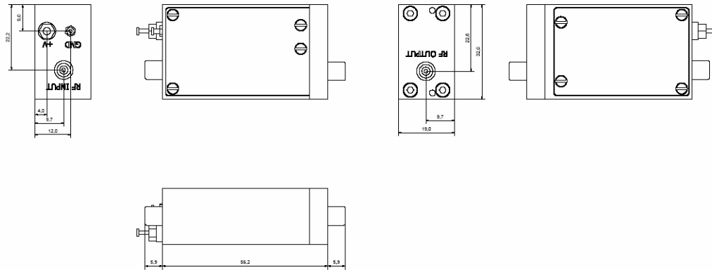
Figure 1. FDA-K outline.
