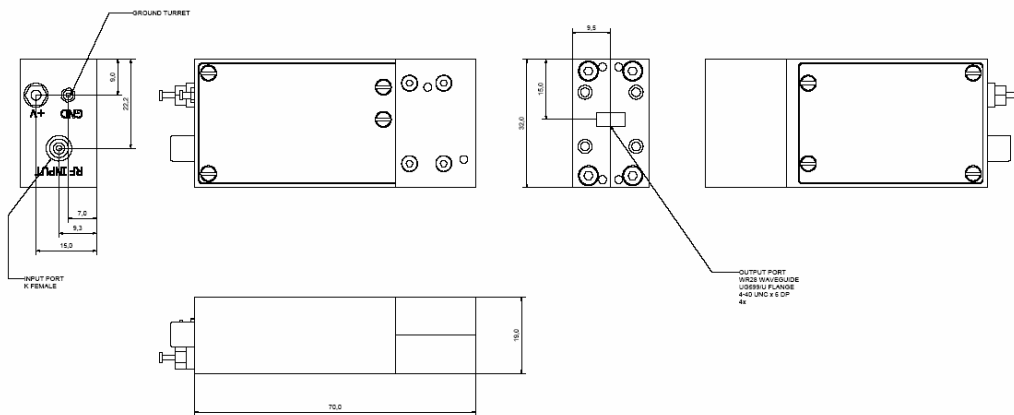
Figure 2. FDA-28 outline.
