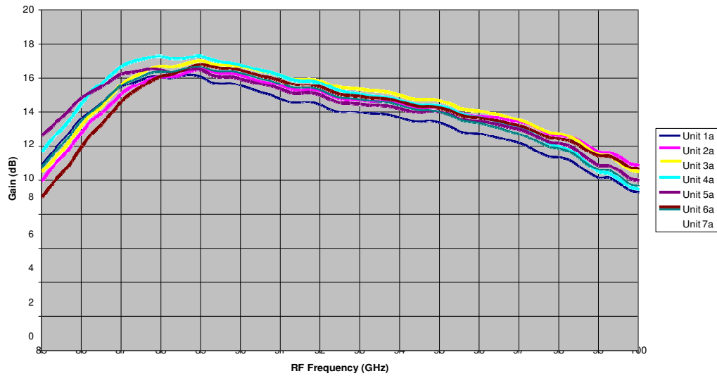
Gain v RF Frequency
