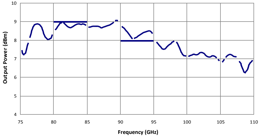
Typical FT-10 Output Power
