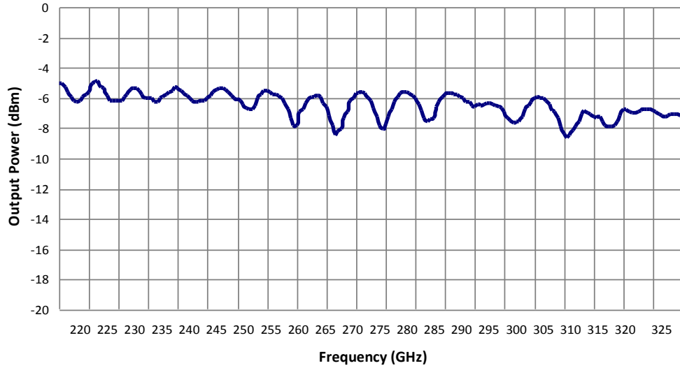
Typical FT-03 Output Power
