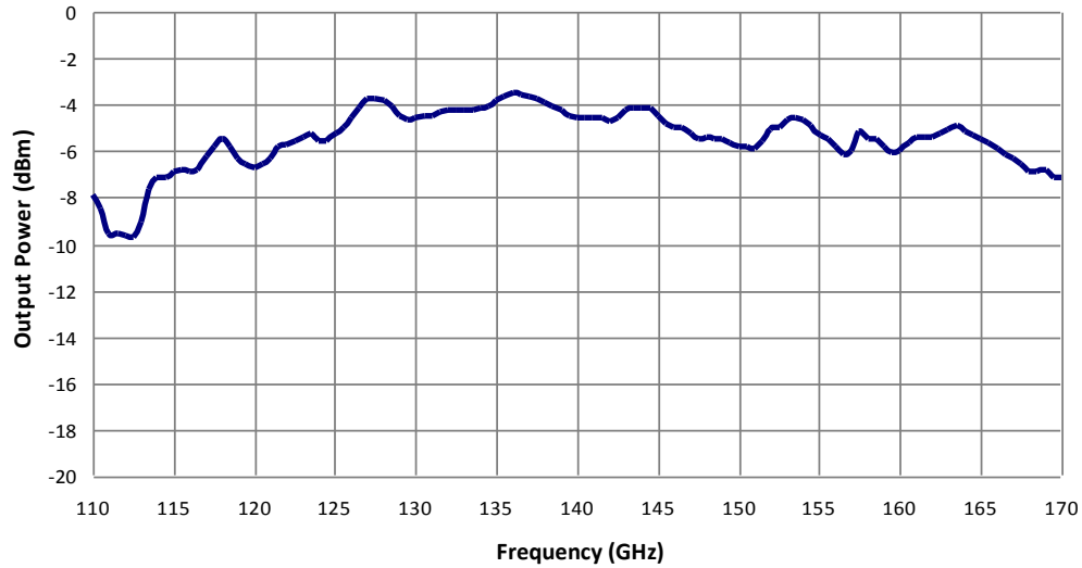
Typical FT-06 Output Power
